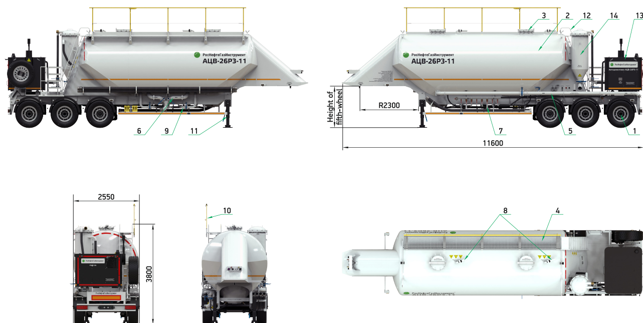
Figure 3 - ACV-26R3-11 bulk cement trailer.
